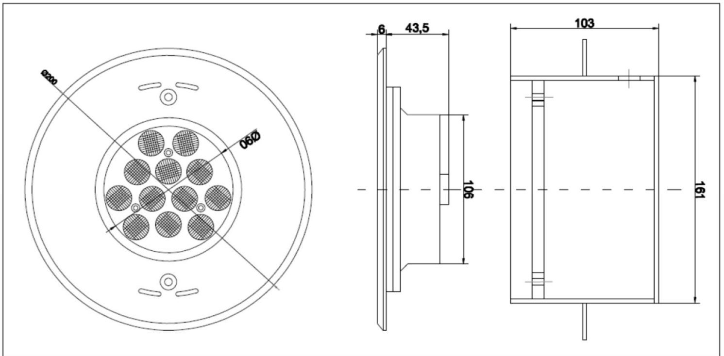
Recess Type
